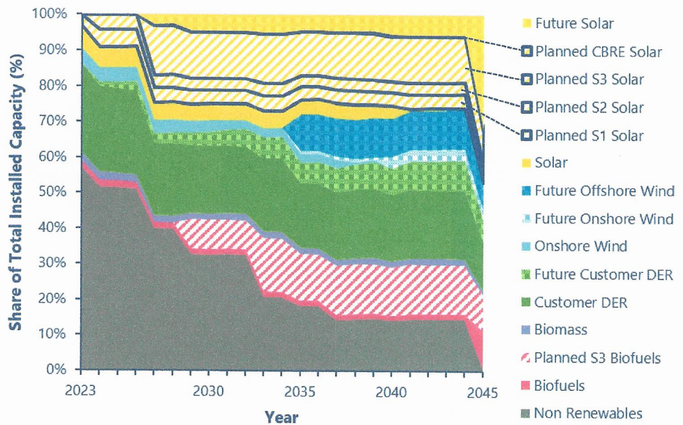
Figure 2-3. O'ahu: Preferred Plan installed capacity mix (2023–2045)
